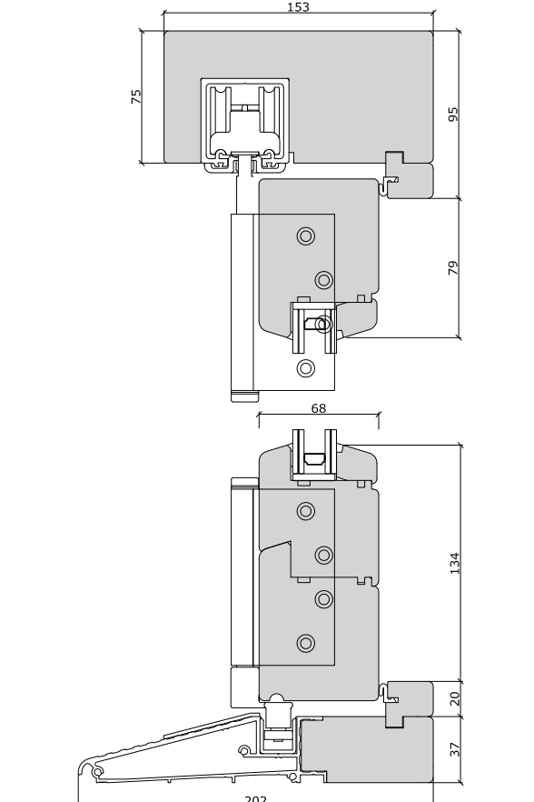
Traditional Range Outward Opening
