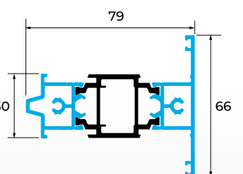
SP210 FLUSH TRANSOM/ MULLION
