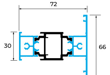
SP200 TRANSOM/ MULLION
