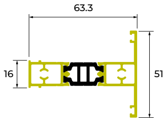
SC200 TRANSOM/MULLION
