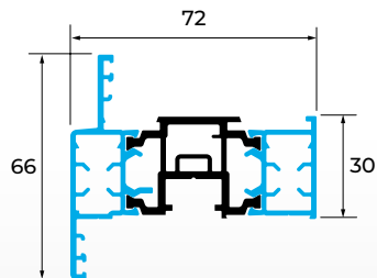
SP301 STEPPED SASH
