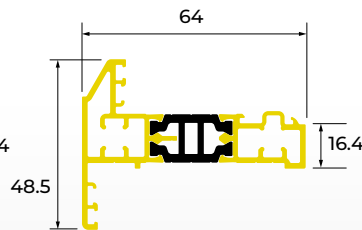
SC315 define BEADED SASH
