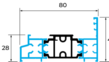
SP101 SMALL FLUSH OUTER FRAME
