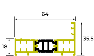
SC100 SMALL OUTER FRAME
