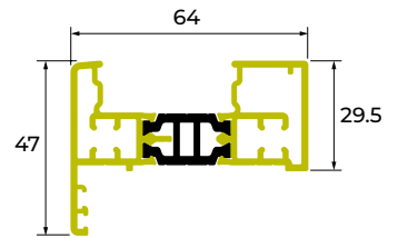
SC301 CONTEMPORARY SASH
