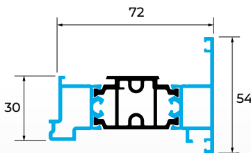
SP250 MEETING STILE
