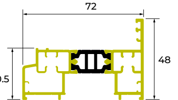
SC103 FLUSH INTERMEDIATE OUTER FRAME
