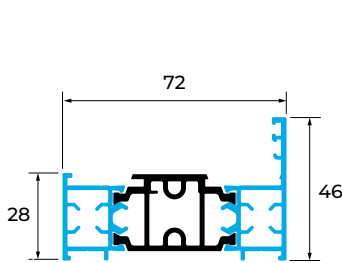
SP100 SMALL OUTER FRAME
