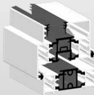
SP403 36mm CLIP-IN BEAD (28mm for stepped sashes)
