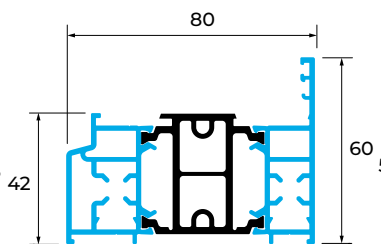
SP103 INTERMEDIATE FLUSH OUTER FRAME
