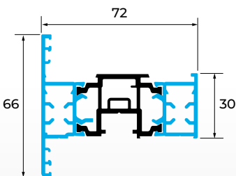
SP301 CONTEMPORARY SASH
