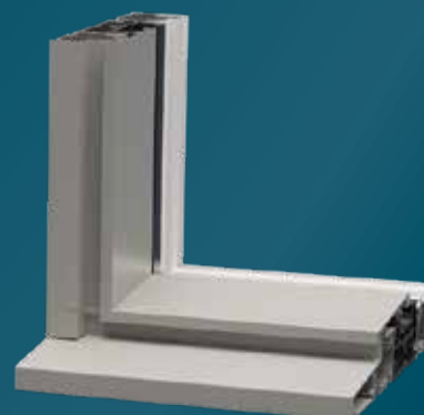
Standard outer frame with clip-on cill nose
