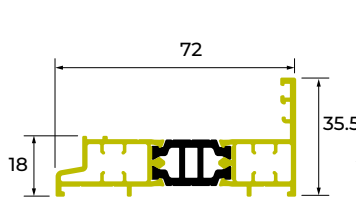
SC101 FLUSH SMALL OUTER FRAME
