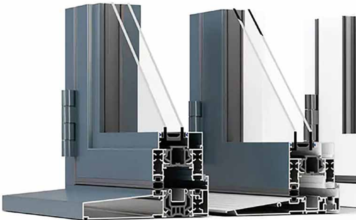
standard cill
