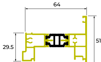
SC250 MEETING STILE
