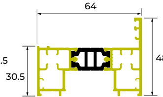
SC102 INTERMEDIATE OUTER FRAME
