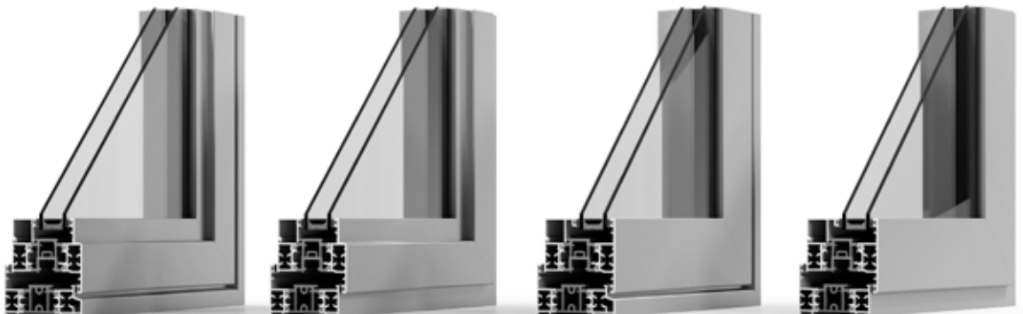
Stepped sash, flush frame
