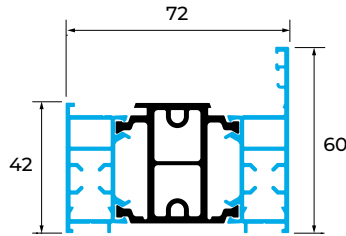
SP102 INTERMEDIATE OUTER FRAME
