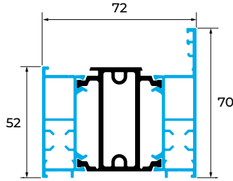
SP104 LARGE OUTER FRAME
