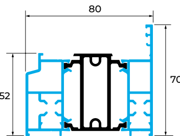
SP105 LARGE FLUSH OUTER FRAME
