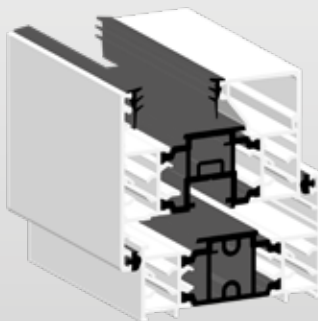
SP401 28mm SHUFFLE BEAD (not for stepped sashes)
